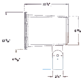
YOKE MOUNT
